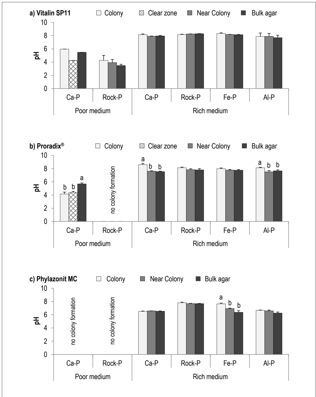
Fig. 4.4: pH values in colonies and their near (3 mm) surrounding (clear zone or near colony) formed by diverse microbial inoculants (a-f) compared to the pH-values far from colonies (bulk agar) after 14 days of cultivation on a poor or rich basal medium supplied with different phosphate forms (Ca-P, Rock-P, Fe-P, or Al-P) in Petri dishes. Columns represent mean values \pm SEM (n = 4). Values of the same treatment group not sharing common letters are significantly different [Tukey's test, p \leq 0.05 ], those without or sharing letters not.
