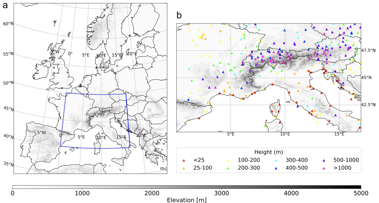
Fig. 1 a EURO-CORDEX full domain, with the common domain across all datasets delimited in blue. b Topography over the common ALP domain, where all computations were carried out. Points refer to
